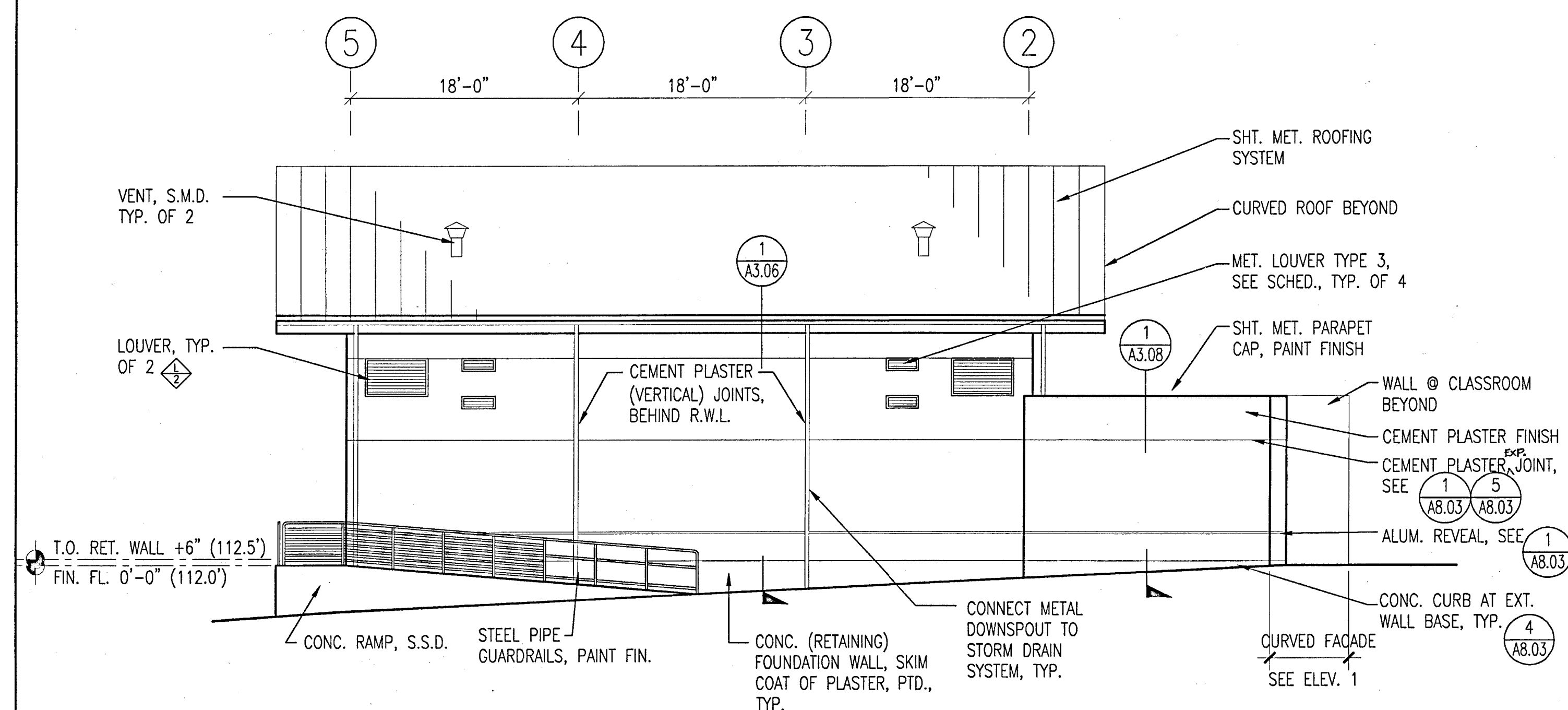
MULTI-PURPOSE BUILDING - EAST ELEVATION 1/8" 2
