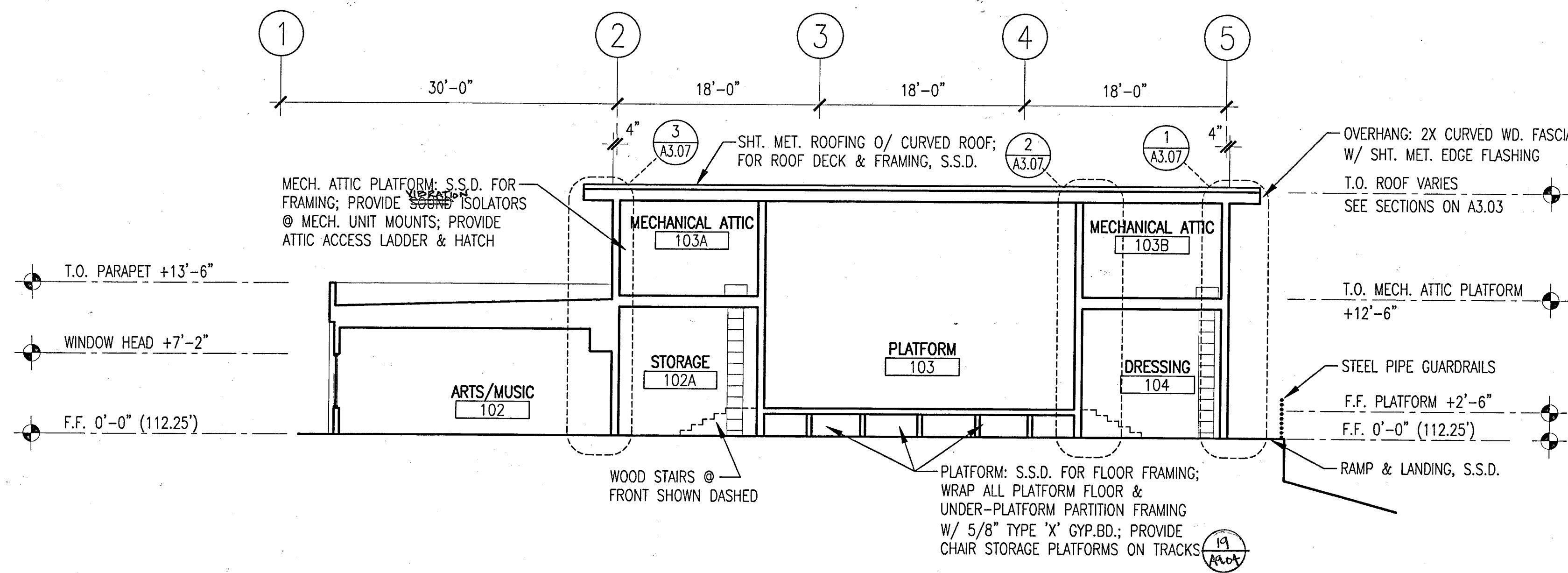
FOR TYP. NOTES, SEE SECTION 2 THIS SHT. MULTI-PURPOSE BUILDING - SECTION 1/8" 1
