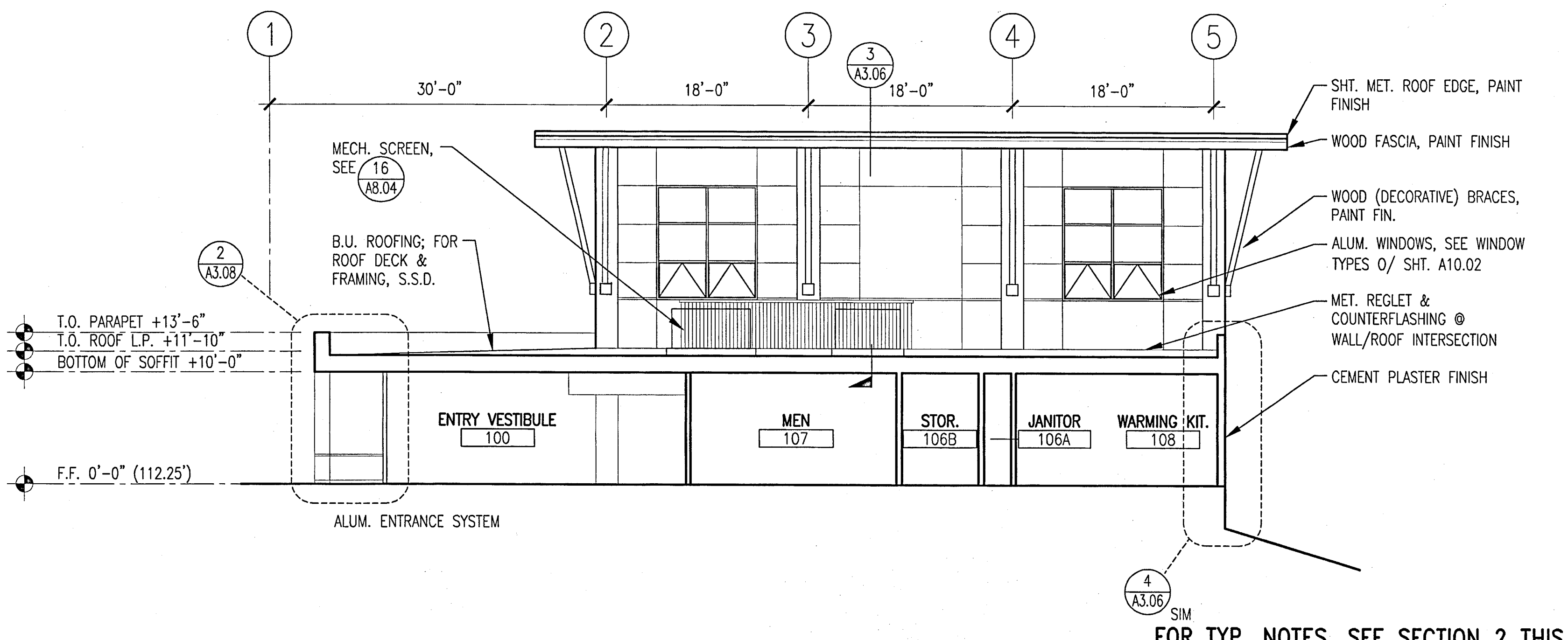
FOR TYP. NOTES, SEE SECTION 2 THIS SHT. MULTI-PURPOSE BUILDING SECTION 1/8" 3
