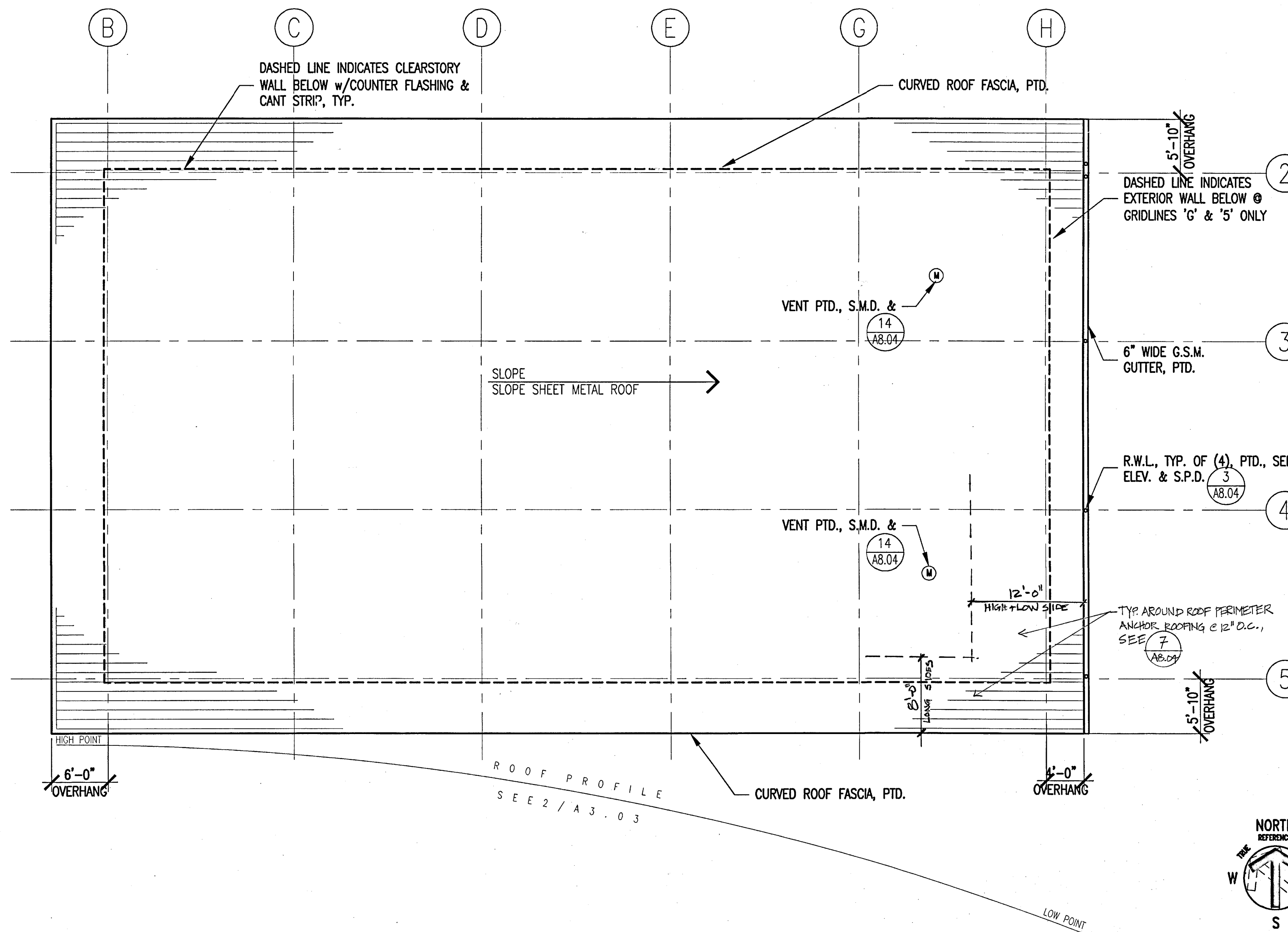
MULTI-PURPOSE, MUSIC & CLASSROOM BUILDING CURVED HIGH ROOF PLAN 1/8" 2
