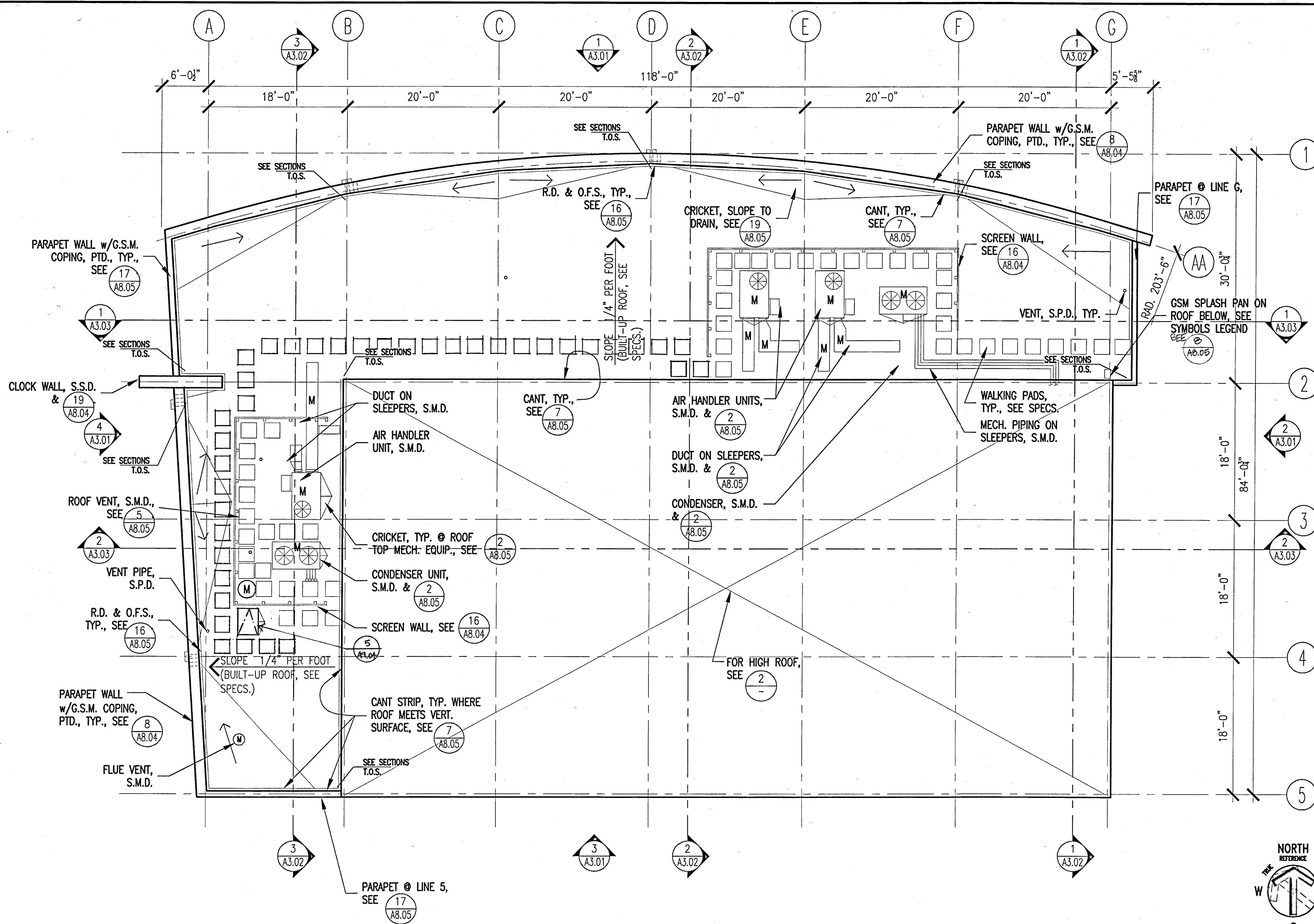
MULTI-PURPOSE, MUSIC & CLASSROOM BUILDING LOW ROOF PLAN 1/8" 1
