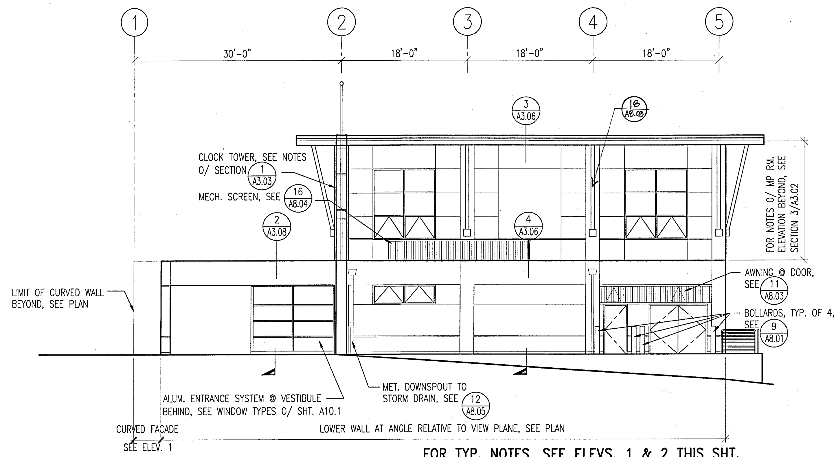
MULTI-PURPOSE BUILDING - WEST ELEVATION 1/8" 4
