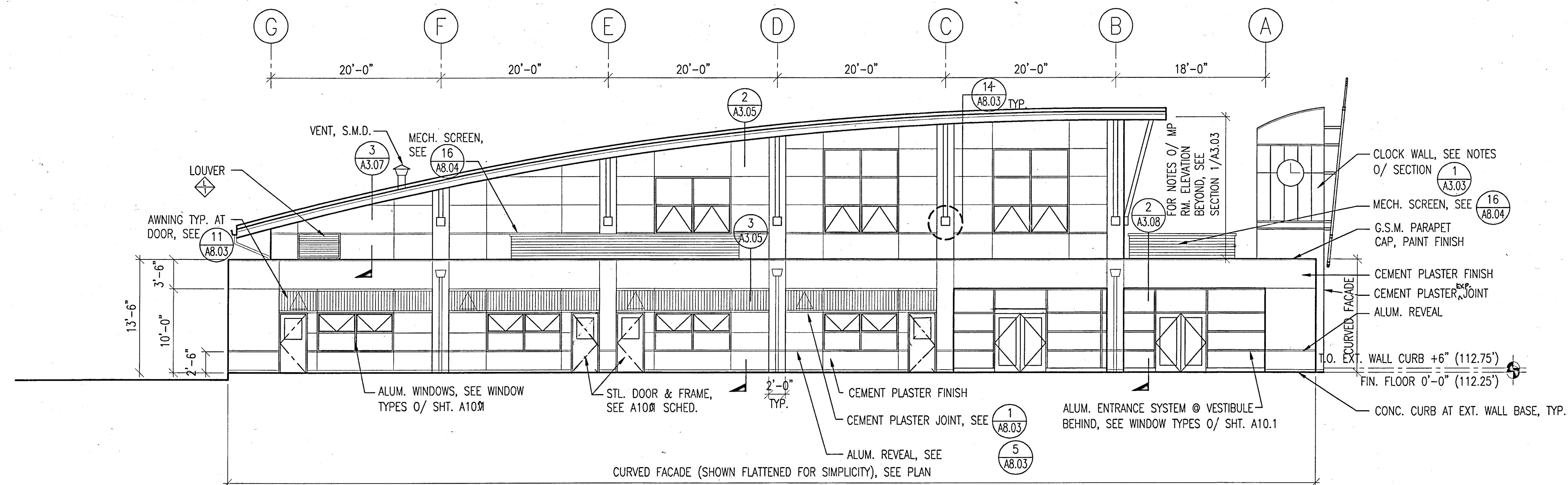
MULTI-PURPOSE BUILDING - NORTH ELEVATION 1/8" 1
