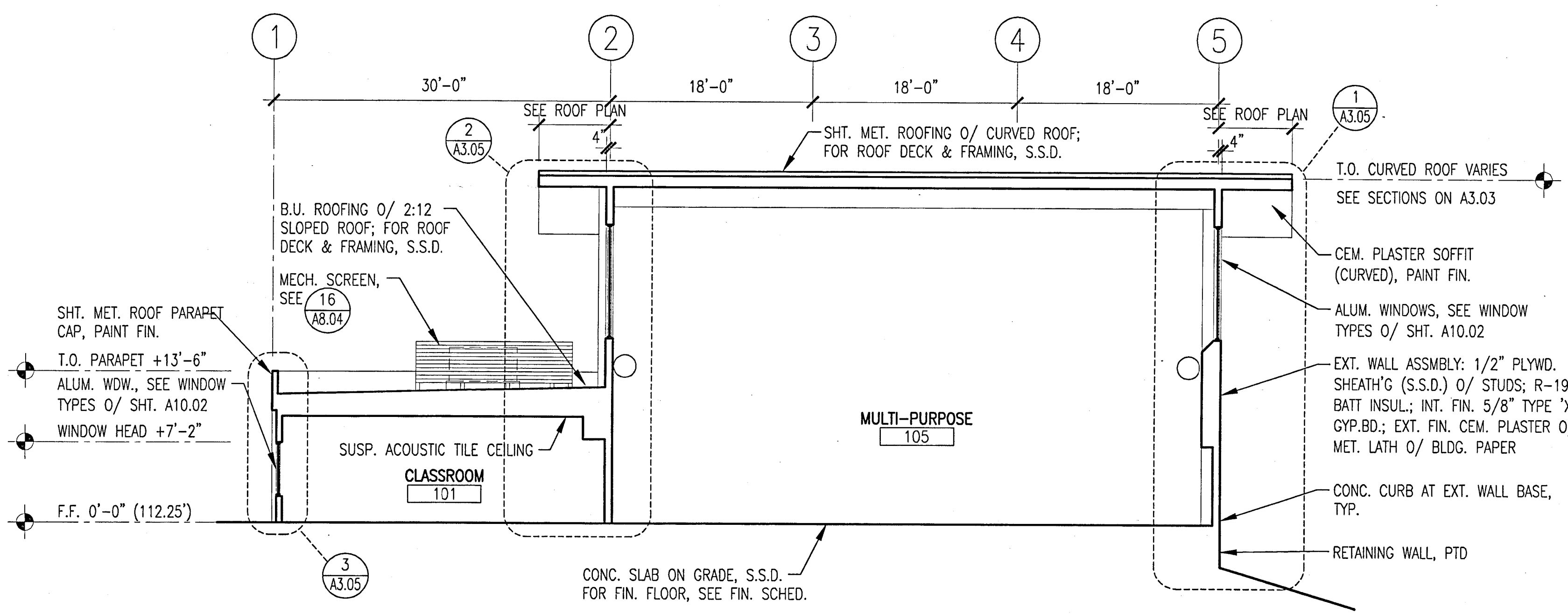
MULTI-PURPOSE BUILDING - SECTION 1/8" 2
